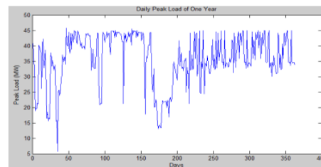
Figure 3. Daily load curve
