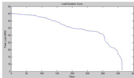
Figure 4. Load duration curve
