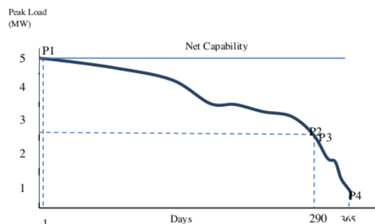
Figure 5. Merging LDC with Probability
